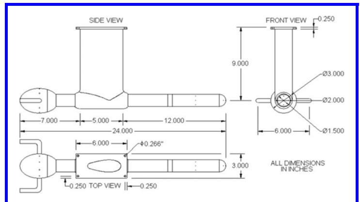
Air Data Probe Physical Dimensions
