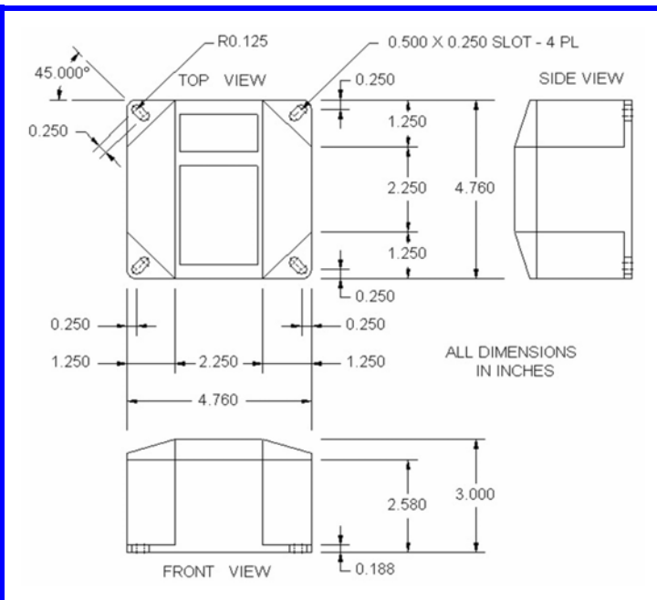
IMU, GPS and CPM Enclosure Physical Dimensions
